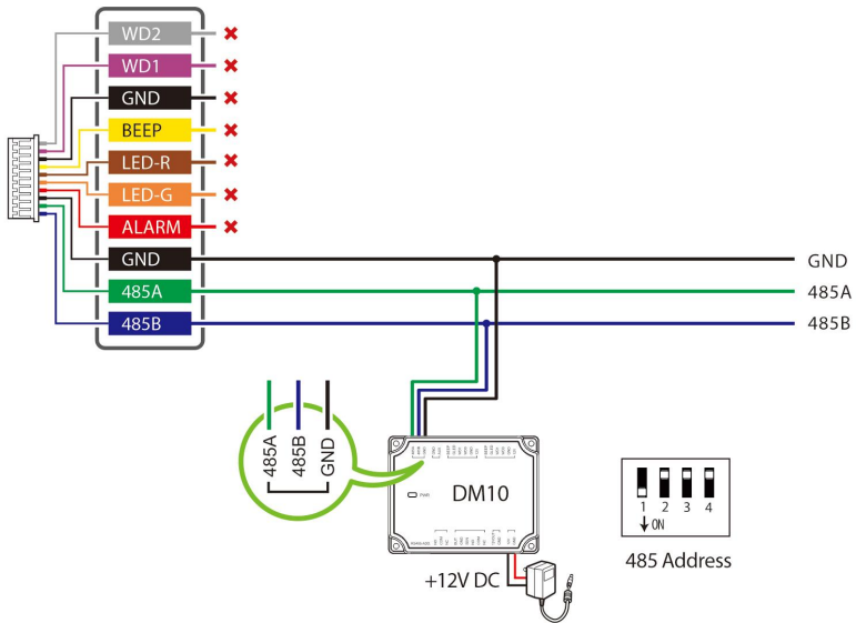
Figure 1-4 DM10 Wiring
