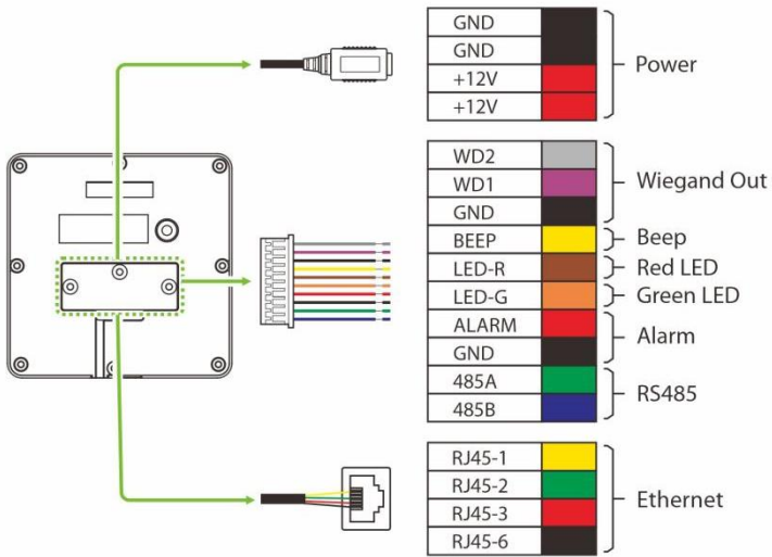
Figure 1-2 Terminal Description
