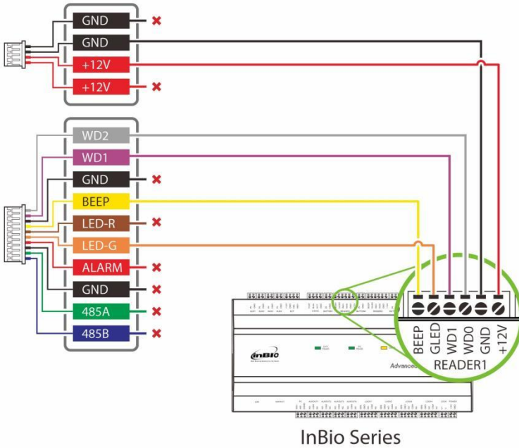
Figure 1-3 InBio Wiring
