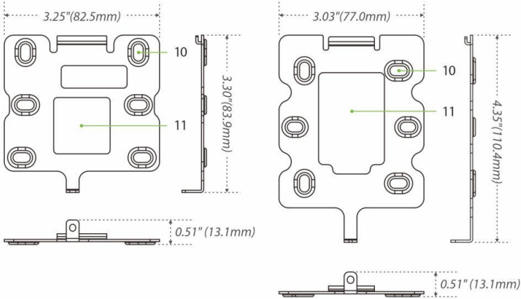
Figure 1-1 KF1100 & KF1200 Appearance
