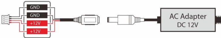
Figure 1-3 Power Wiring
