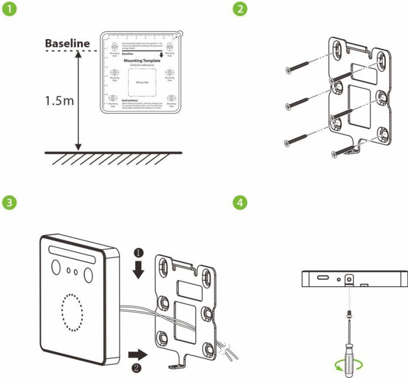
Figure1-5 KF1000 Series Installation
